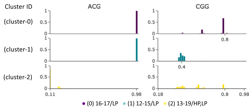
Fig. 13. Codons separating clusters (H7N9). Distribution of RSCUs (exp. value = 1) for codons ACG and CGG (i.e., those for which RSCU distribution mostly differs among the 3 clusters). See boxplot in the Supplementary File, Fig. S11.
