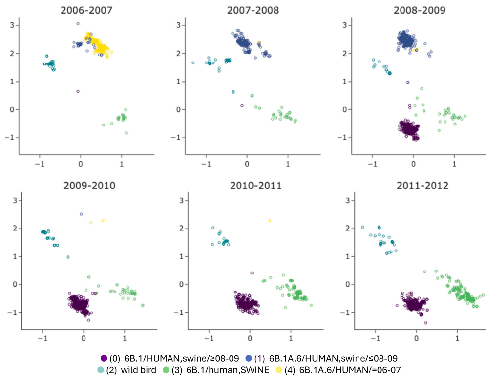
Fig. 4. Codon profiles of clusters (H1N1). The codon profile of the H1N1 sequences is projected on the PC1 (y-axis) and PC3 (x-axis). The scatter plot is organized by flu season. Each sequence is colored according to the assigned cluster.
