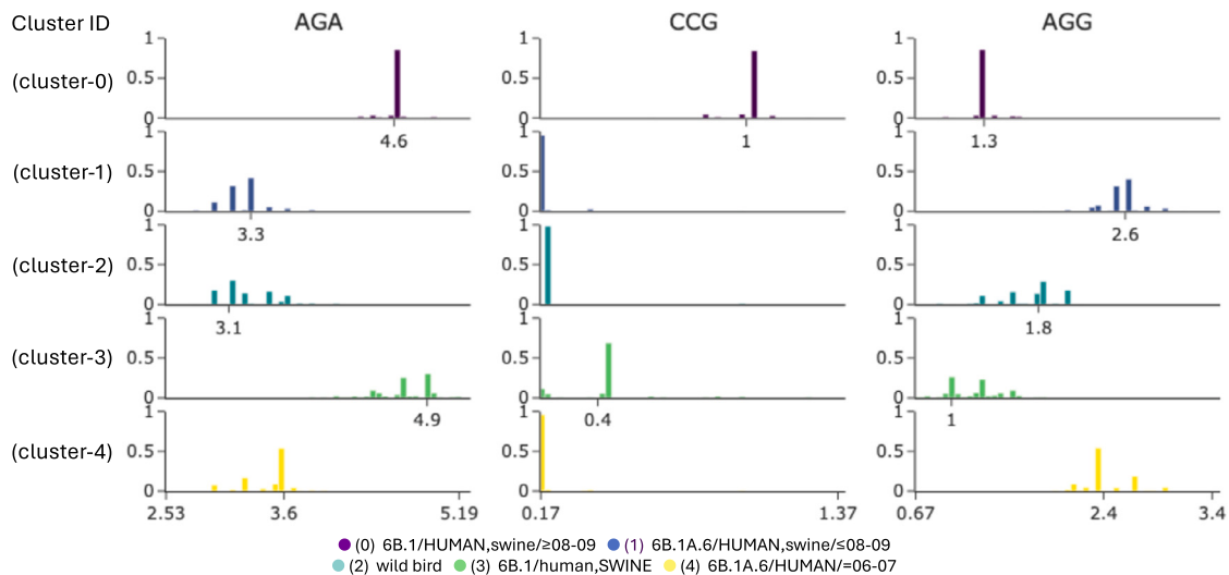
Fig. 12. Codons separating clusters (H1N1). Distribution of RSCUs (exp. value = 1) for codons AGA, CCG, and AGG (i.e., codons for which RSCU distribution mostly differs between the 5 clusters). See boxplot in the Supplementary File, Fig. S10.
