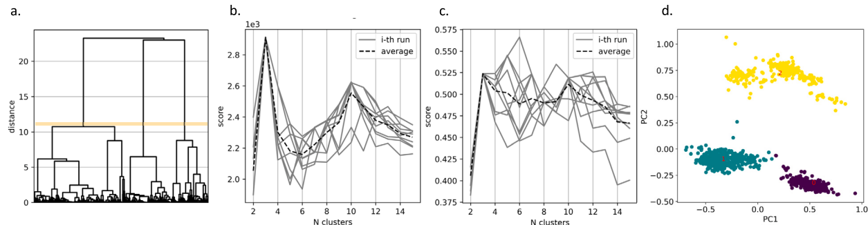
Fig. 6. Clustering (H7N9). a) Dendrogram of the agglomerative clustering algorithm on the H7N9 dataset; b) Calinski-Harabasz scores of the 10-fold k-means clustering algorithm; c) Silhouette scores of the 10-fold k-means clustering algorithm; d) Clusters of sequences highlighted using different colors and plotted on the PC1 and PC2.
