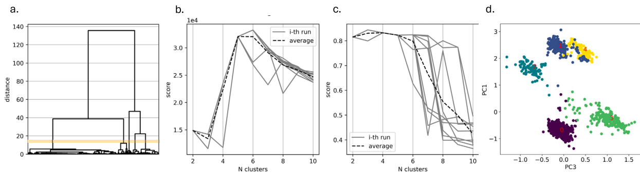
Fig. 3. Clustering (H1N1). a) Dendrogram of the agglomerative clustering algorithm on the H1N1 dataset; b) Calinski-Harabasz scores of the 10-fold k-means clustering algorithm; c) Silhouette scores of the 10-fold k-means clustering algorithm; d) Clusters of sequences highlighted using different colors and plotted on the PC1 and PC3.
