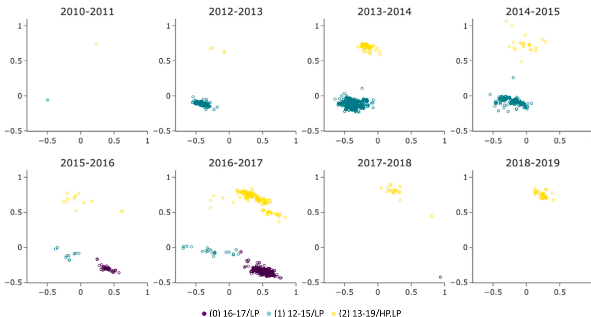
Fig. 7. Codon profiles of clusters (H7N9). The codon profile of the H7N9 sequences is projected on the PC1 (x-axis) and PC2 (y-axis). The scatter plot is organized by flu season. Each sequence is colored according to the assigned cluster.
