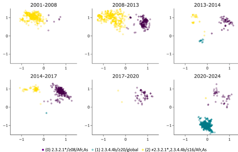
Fig. 10. Codon profiles of clusters (H5N1). The codon profile of the H5N1 sequences is projected on the PC2 (x-axis) and PC1 (y-axis). The scatter plot is organized by flu season. Each sequence is colored according to the assigned cluster.
