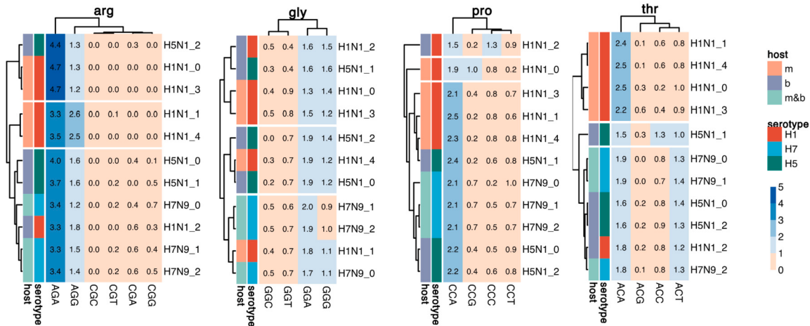
Fig. 11. Average RSCU values for all the synonymous codons of the four most informative amino acids. Each heatmap shows, on a color scale from pink (low) to dark blue (high) blue, the RSCU values for all the synonymous codons of selected amino acids. Each row represents the values of one of the possible codons encoding the amino acid, in one of the clusters defined by our approach in three use cases (H1N1, H7N9, and H5N1). Bars on the left are used to indicate the serotype and host (m = mammals, b = birds, m&b = mammal and birds) according to the color code in the legend, for every cluster.
