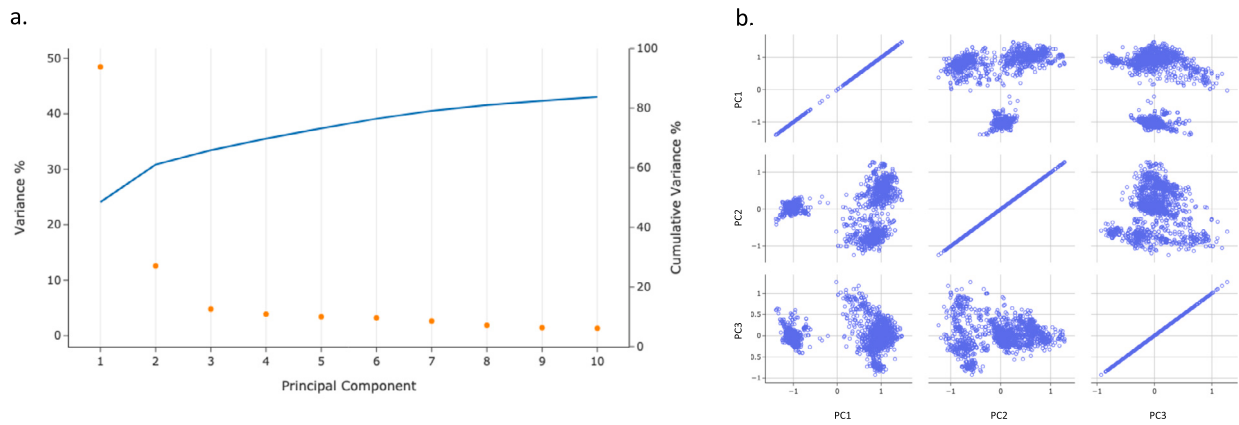
Fig. 8. Principal Components Analysis (H5N1). a) Elbow plot of the PC. In blue, the cumulative explained variance, in red the variance explained by every single component. b) Scatter matrix of the dataset projected on the first 3 PCs.
