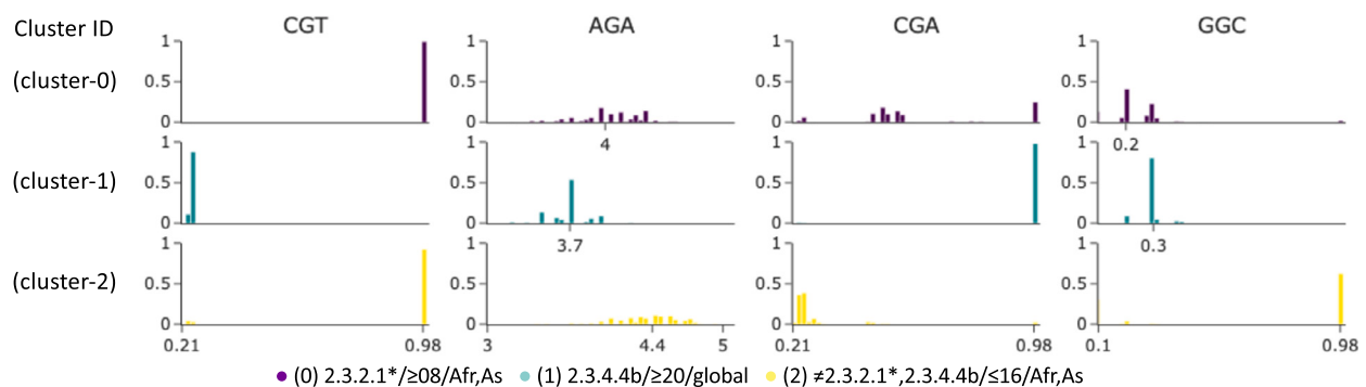
Fig. 14. Codons separating clusters (H5N1). Distribution of RSCUs (exp. value = 1) for four codons CGT, AGA, CGA, and GGC, for which RSCU distribution mostly differs among the 3 clusters. See the boxplot in the Supplementary File, Fig. S12. Corresponding charts for the H5N1 wild birds case are reported in the Supplementary File, Figs. S13–S14.
