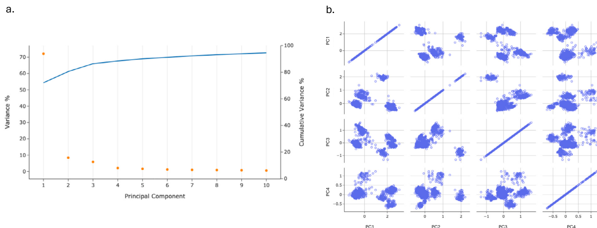
Fig. 2. Principal Components Analysis (H1N1). a) Elbow plot of the PCs. In blue is the cumulative explained variance, and in red is the variance explained by every single component. b) Scatter matrix of the dataset projected on the first 4 PCs.
