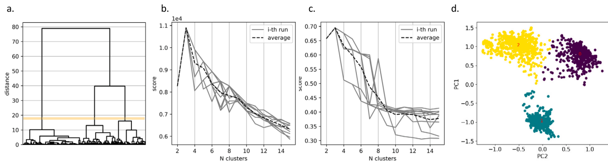
Fig. 9. Clustering (H5N1). a) Dendrogram of the agglomerative clustering algorithm on the H5N1 dataset; b) Calinski-Harabasz scores of the 10-fold k-means clustering algorithm; c) Silhouette scores of the 10-fold k-means clustering algorithm; d) Clusters of sequences highlighted using different colors and plotted on the PC1 and PC2.
