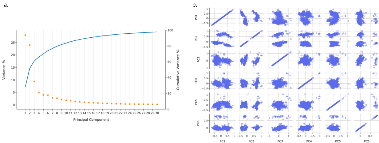
Fig. 5. Principal Components Analysis (H7N9). a) Elbow plot of the PCs. In blue, the cumulative explained variance, in red the variance explained by every single component. b) Scatter matrix of the dataset projected on the first 6 PCs.
