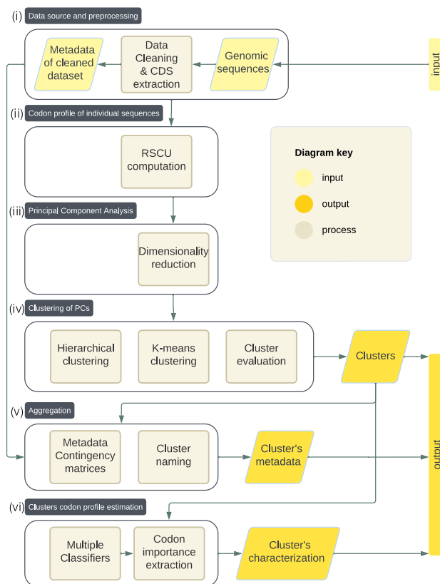
Fig. 1. Schematic overview of methods. We (i) preprocess genomic data and metadata; (ii) compute RSCU values for all the sequences; (iii) run PCA analysis; (iv) cluster along the Principal Components and select the most appropriate number of clusters; (v) assign interpretable labels to clusters; and (vi) characterize clusters by their most important codons.
